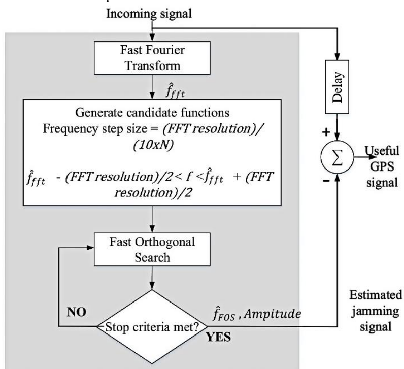
Figure 2. Flowchart of the anti-jamming technique proposed in [10].
